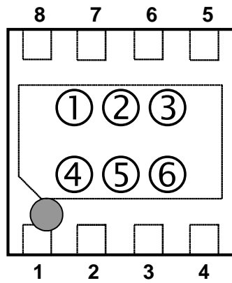
DFN (PLP) 2020-8 Part Markings
