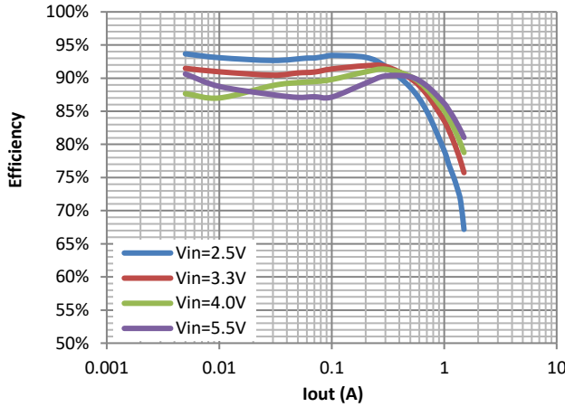
Efficiency vs. Output Current ( V_{out}=1.8\text{V} )
