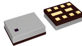
HFFP10-JL 1.57 x 1.23 mm typ., t = 0.47 mm max.
